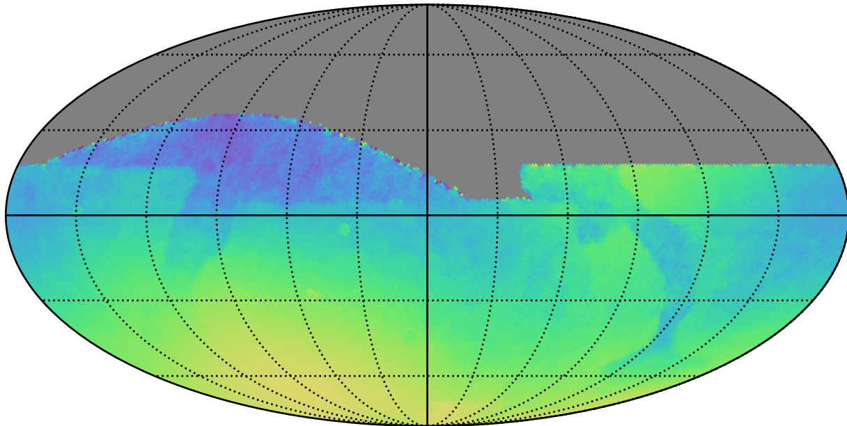
baseline_v2.0_10yrs All sky: Normalized Parallax Uncert @ 22.4
