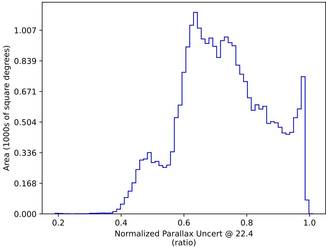
baseline_v2.0_10yrs All sky: Normalized Parallax Uncert @ 22.4
