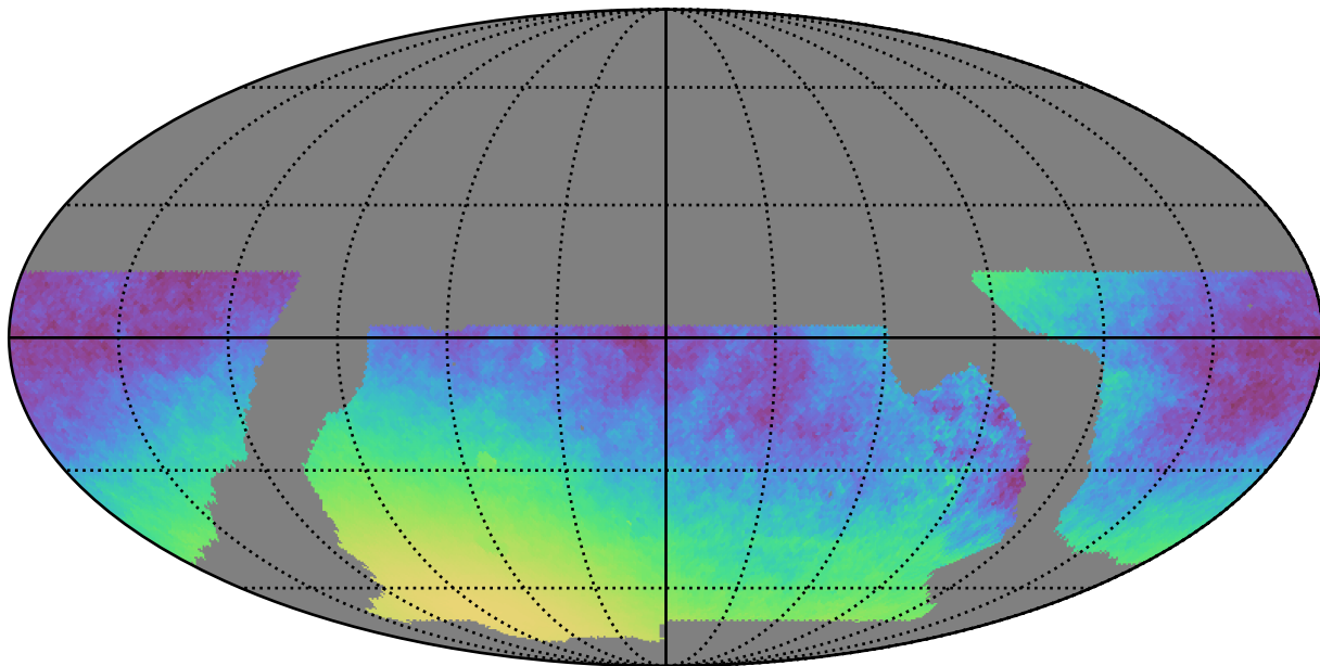
baseline_v2.0_10yrs WFD y band only: Normalized Parallax Uncert @ 21.3
