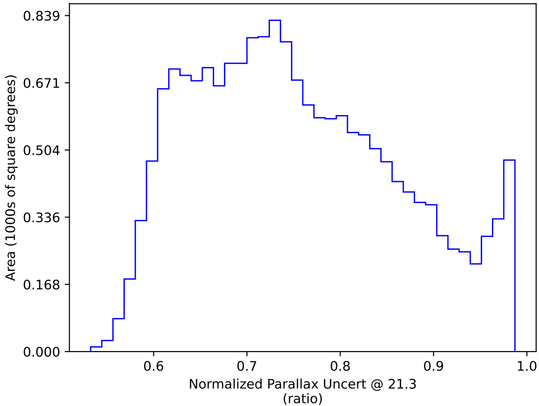
baseline_v2.0_10yrs WFD y band only: Normalized Parallax Uncert @ 21.3
