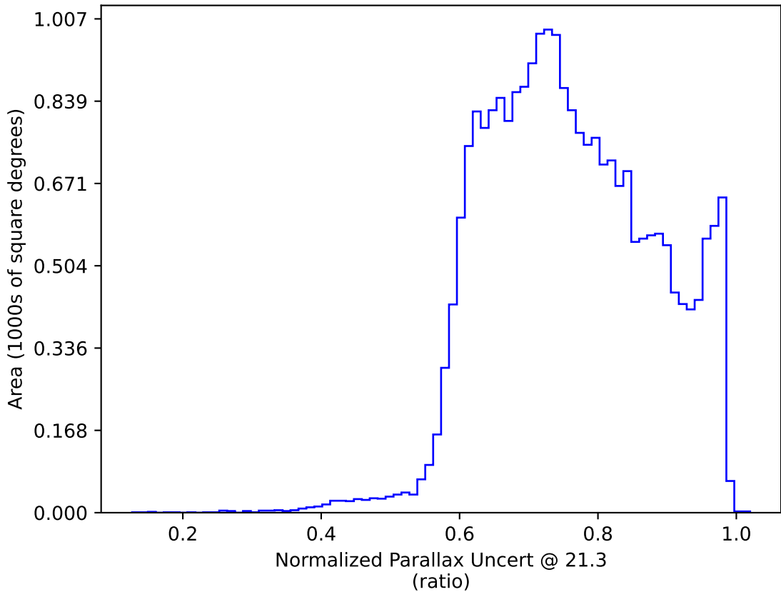
baseline_v2.0_10yrs All sky y band only: Normalized Parallax Uncert @ 21.3
