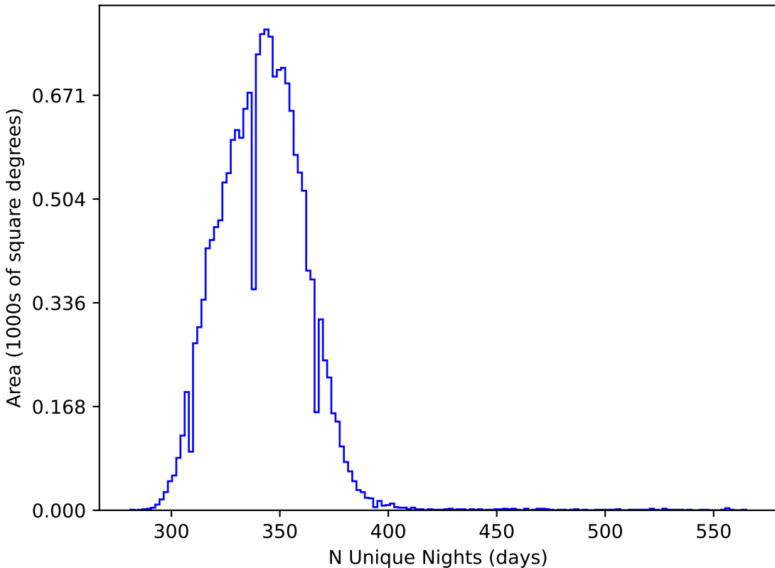
baseline_v2.0_10yrs WFD all bands: N Unique Nights
