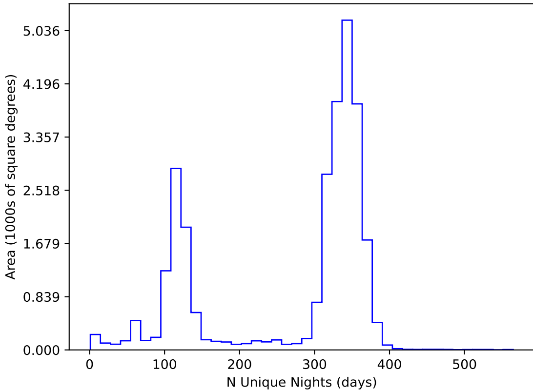
baseline_v2.0_10yrs All sky all bands: N Unique Nights
