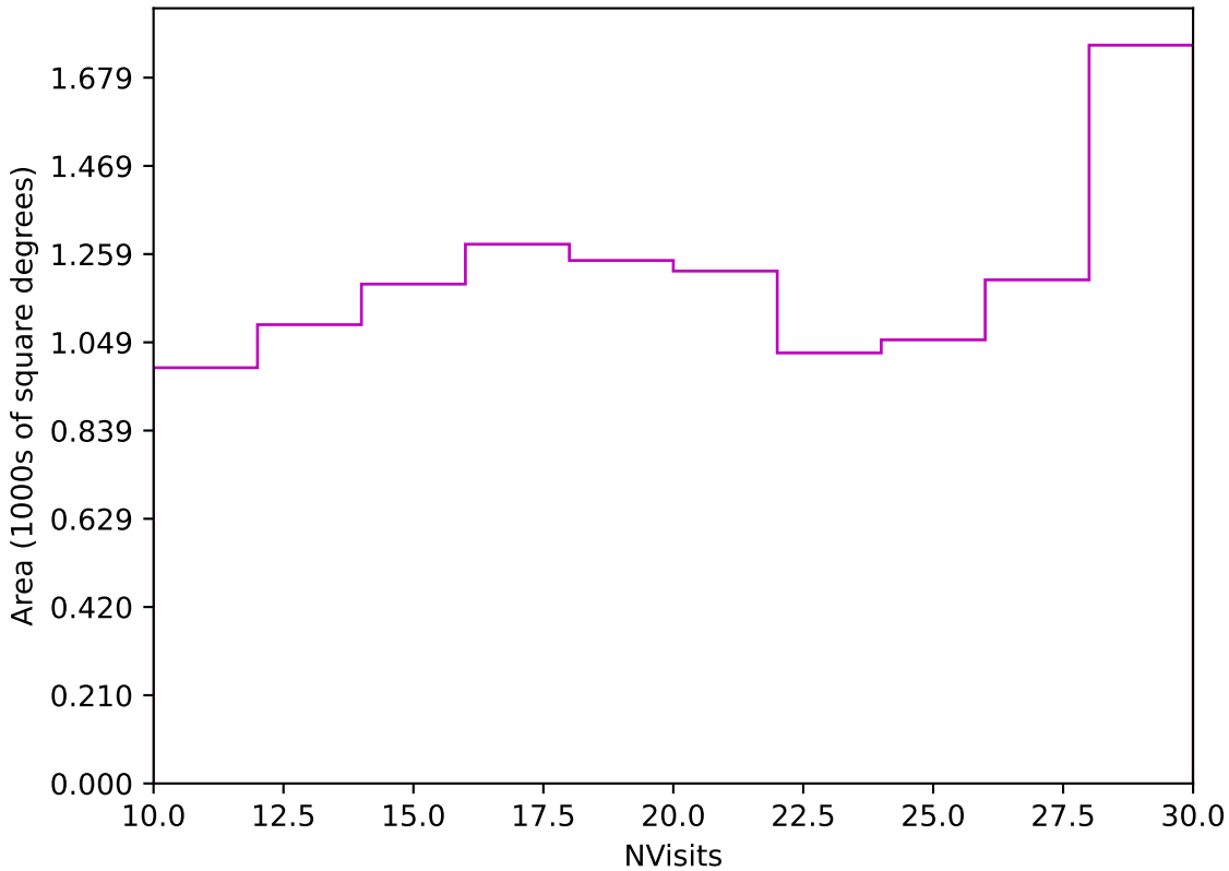
baseline_v2.0_10yrs Yr 3-4 z band: NVisits
