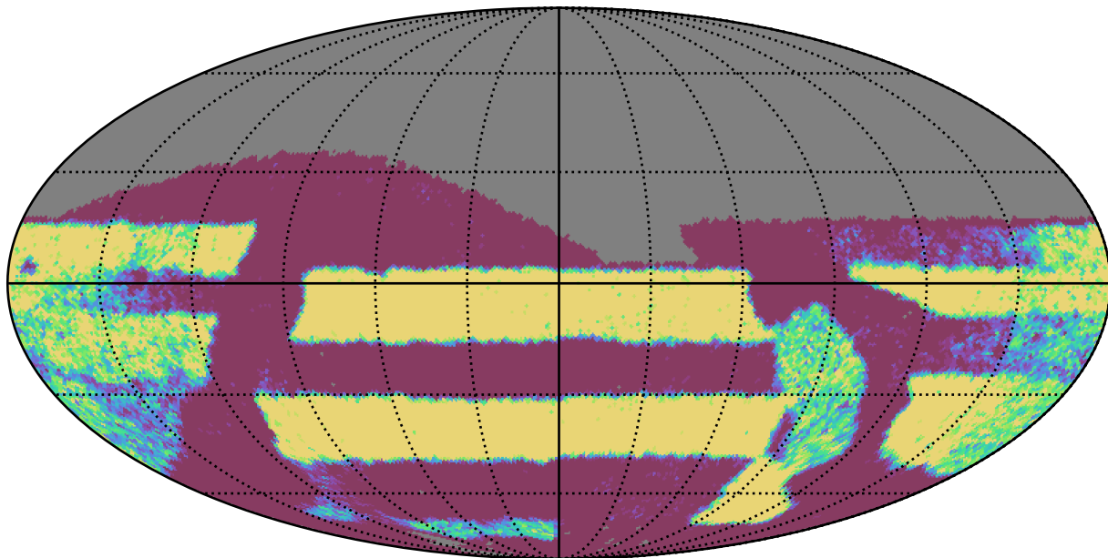
baseline_v2.0_10yrs Yr 3-4 r band: NVisits
