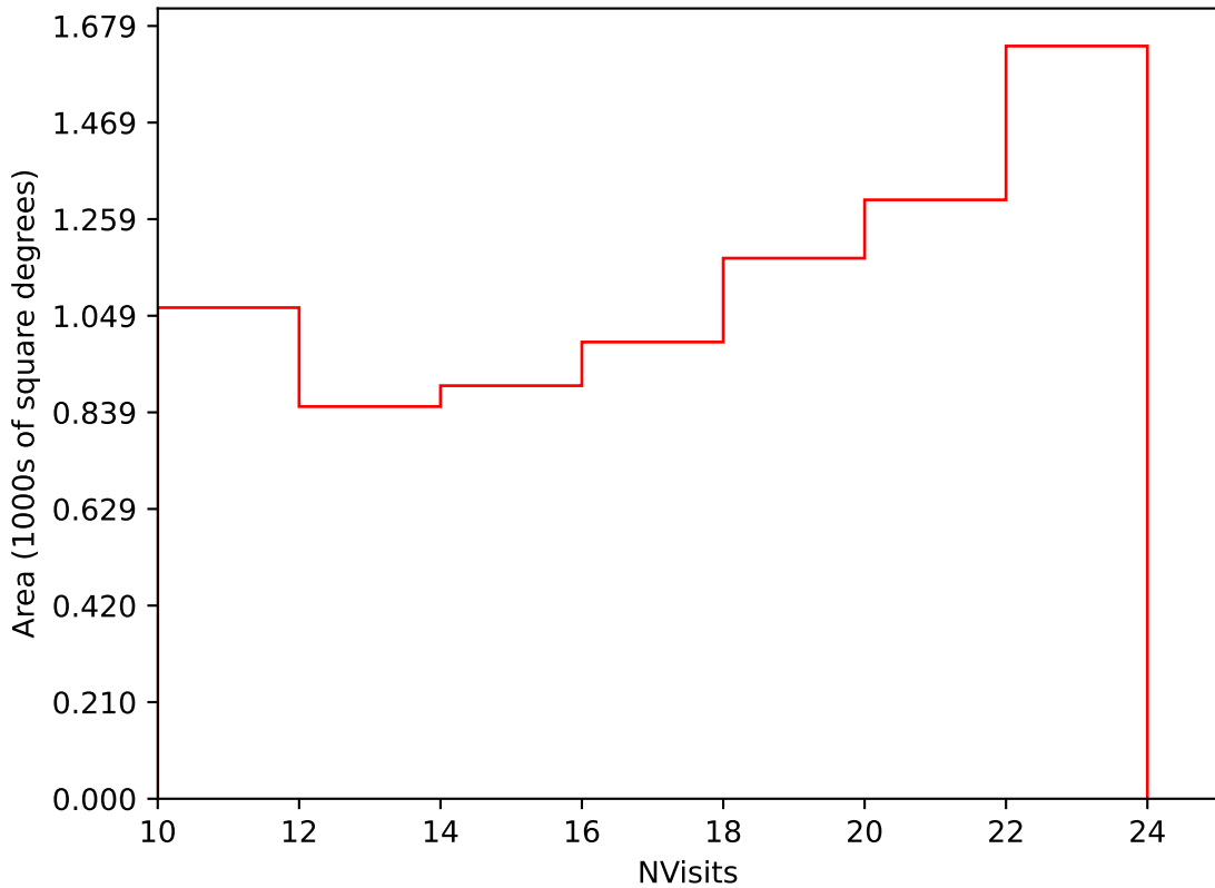
baseline_v2.0_10yrs Yr 3-4 i band: NVisits
