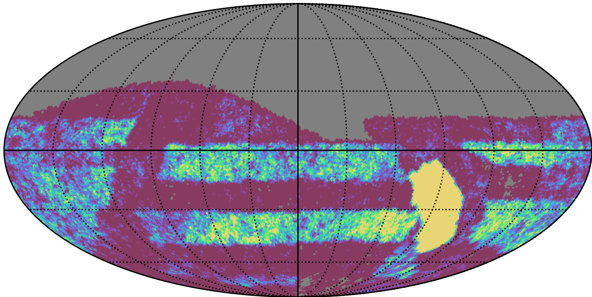
baseline_v2.0_10yrs Yr 3-4 g band: NVisits
