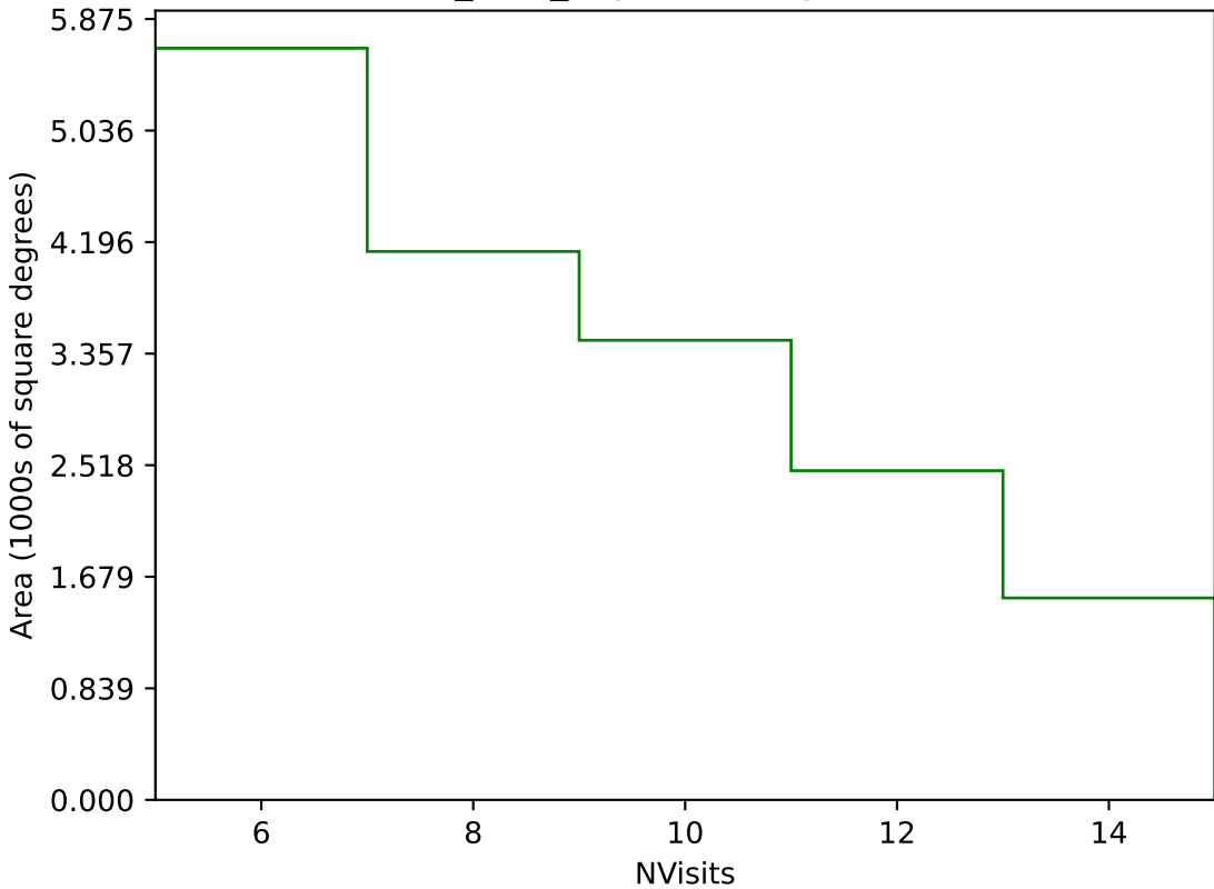
baseline_v2.0_10yrs Yr 3-4 g band: NVisits
