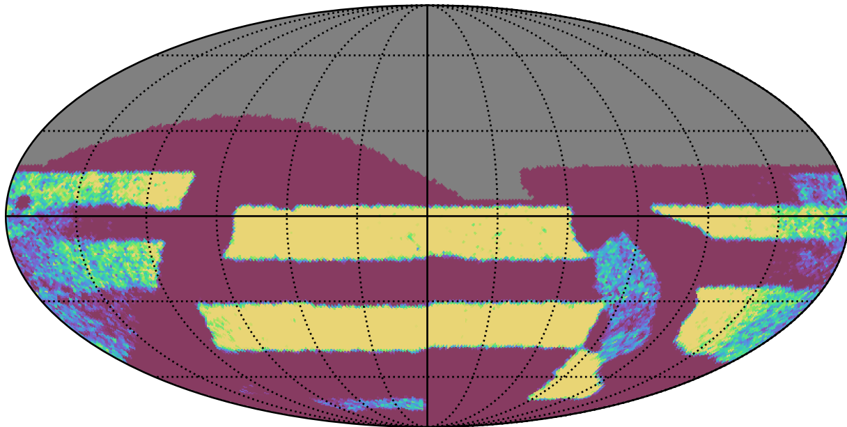
baseline_v2.0_10yrs Yr 3-4 all bands: NVisits
