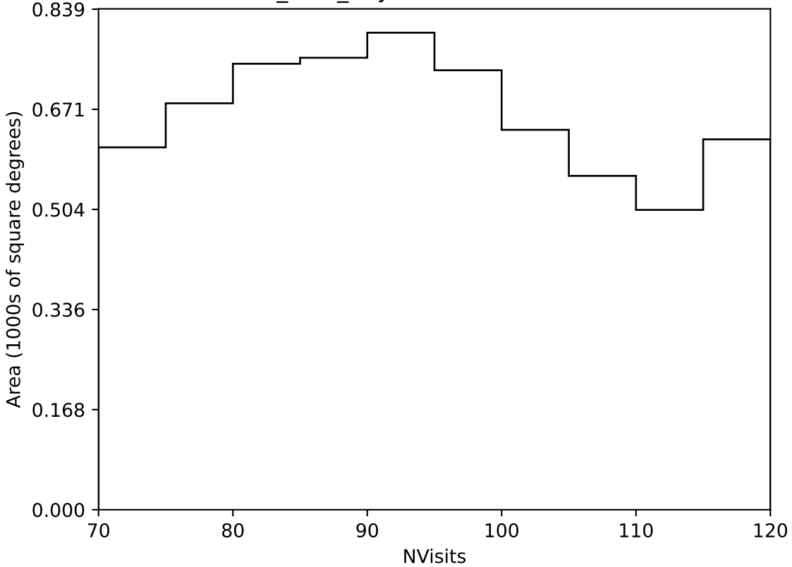
baseline_v2.0_10yrs Yr 3-4 all bands: NVisits
