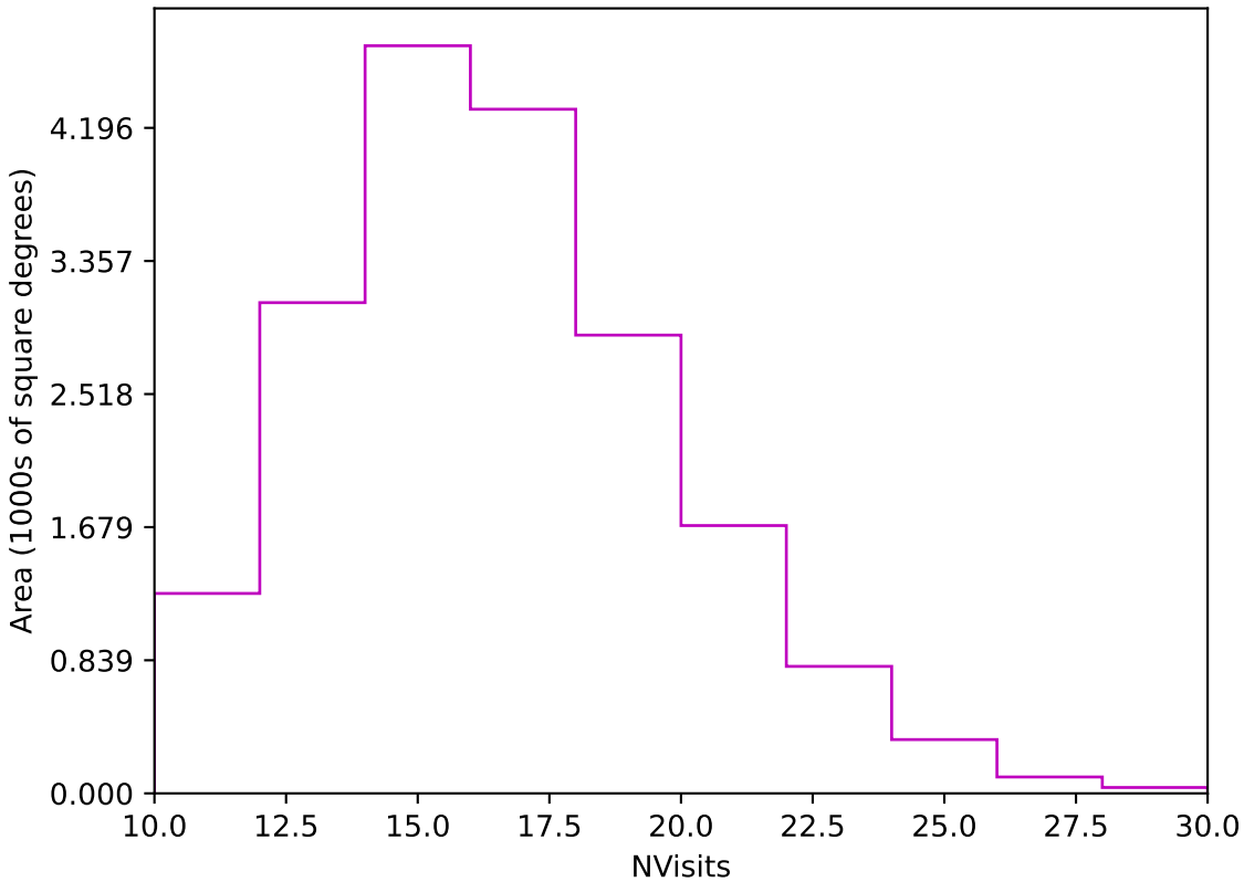
baseline_v2.0_10yrs Yr 1 z band: NVisits
