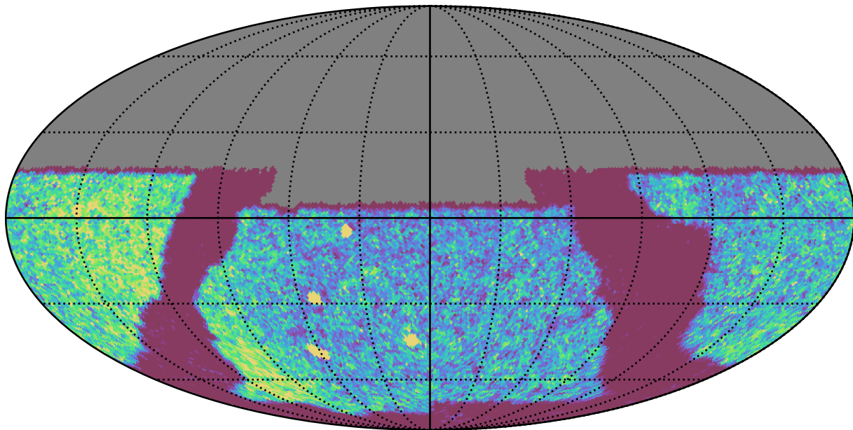
baseline_v2.0_10yrs Yr 1 y band: NVisits
