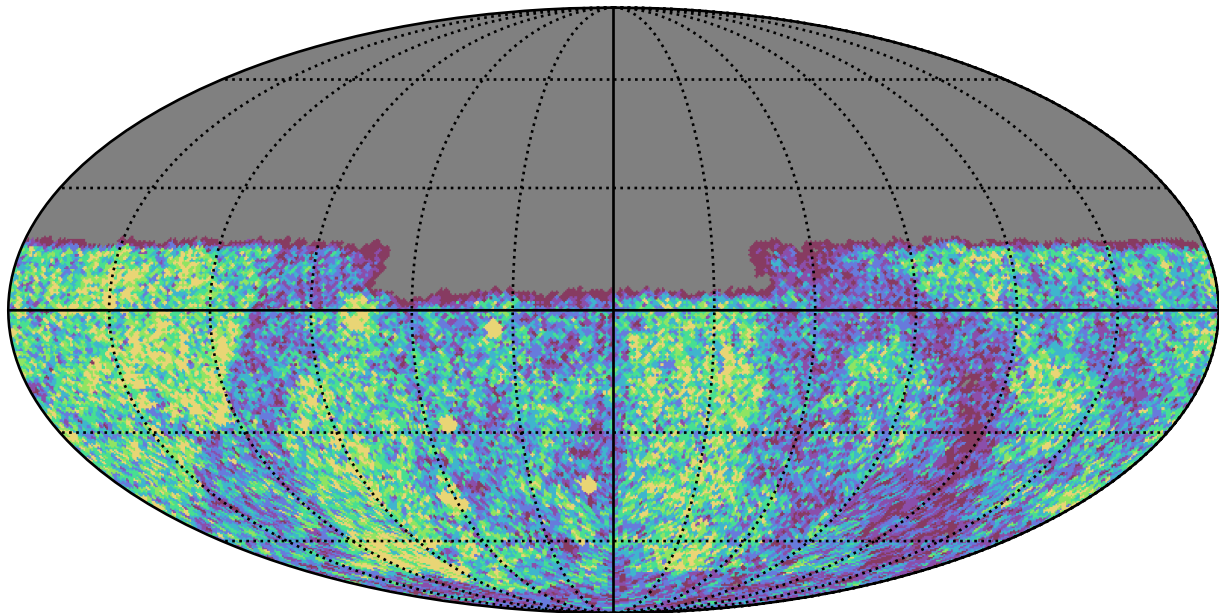
baseline_v2.0_10yrs Yr 1 u band: NVisits
