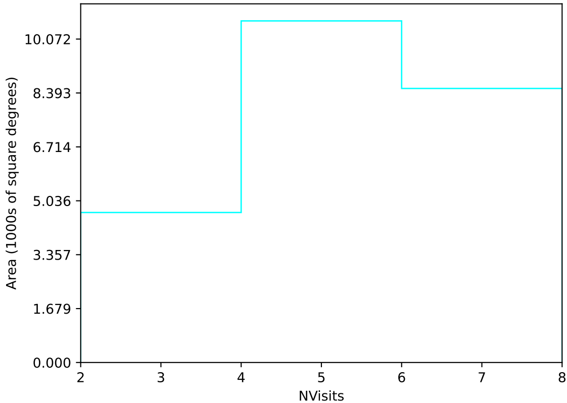
baseline_v2.0_10yrs Yr 1 u band: NVisits
