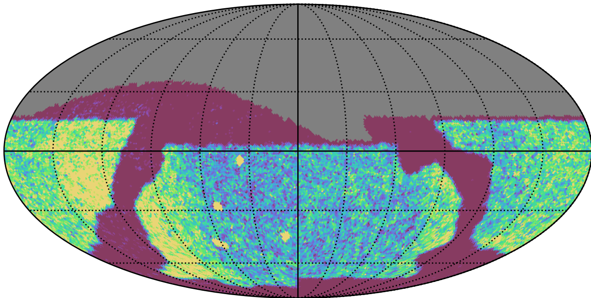
baseline_v2.0_10yrs Yr 1 i band: NVisits
