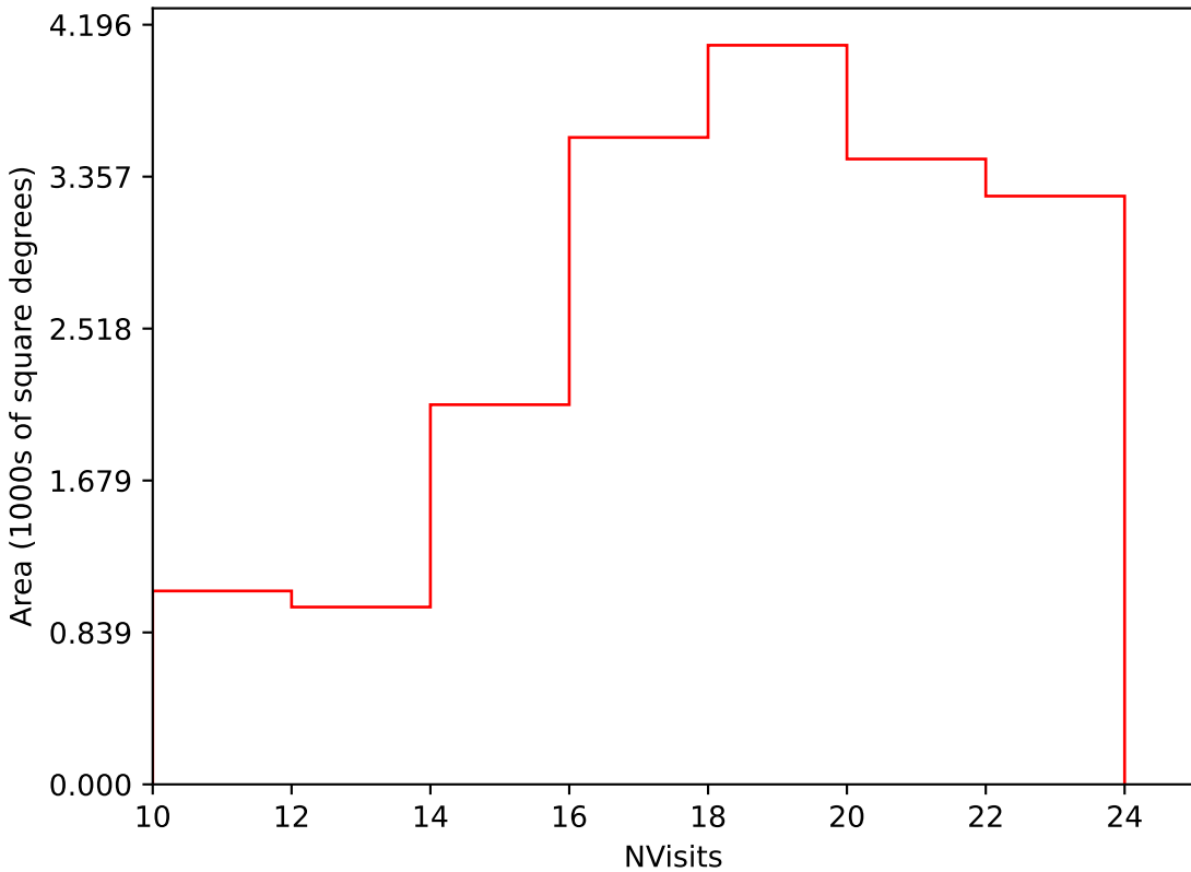
baseline_v2.0_10yrs Yr 1 i band: NVisits
