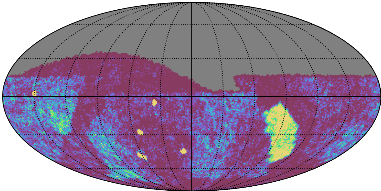
baseline_v2.0_10yrs Yr 1 g band: NVisits
