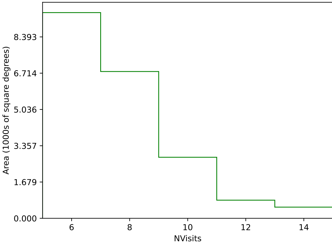
baseline_v2.0_10yrs Yr 1 g band: NVisits
