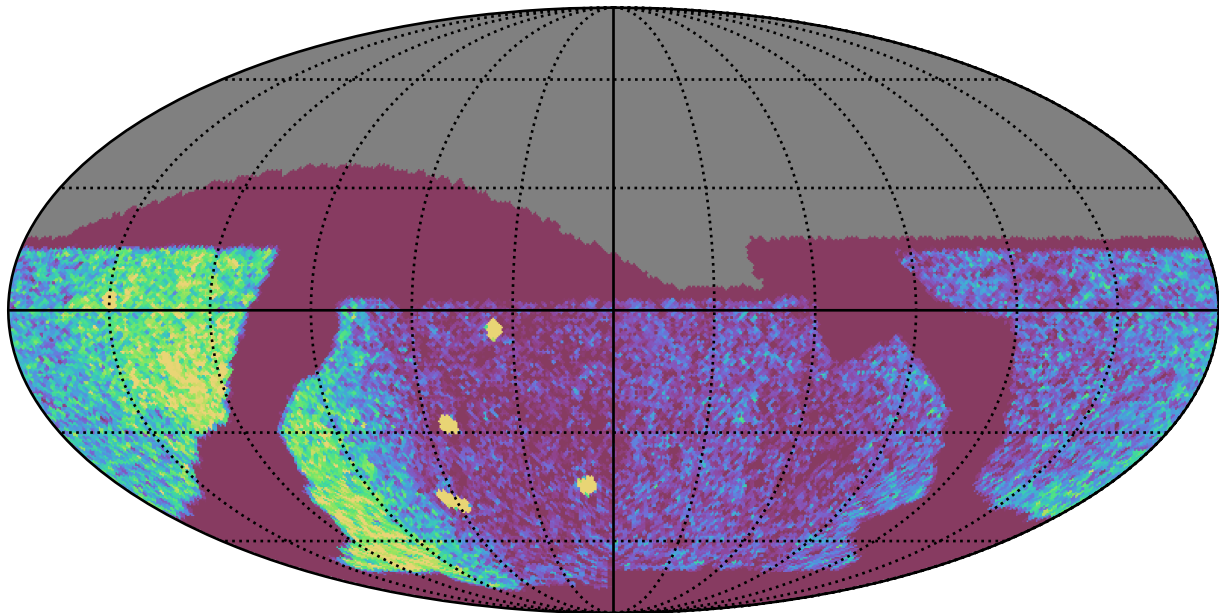
baseline_v2.0_10yrs Yr 1 all bands: NVisits
