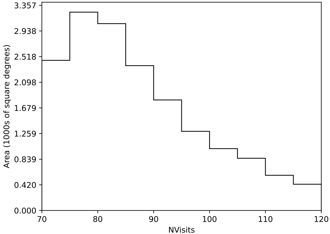
baseline_v2.0_10yrs Yr 1 all bands: NVisits
