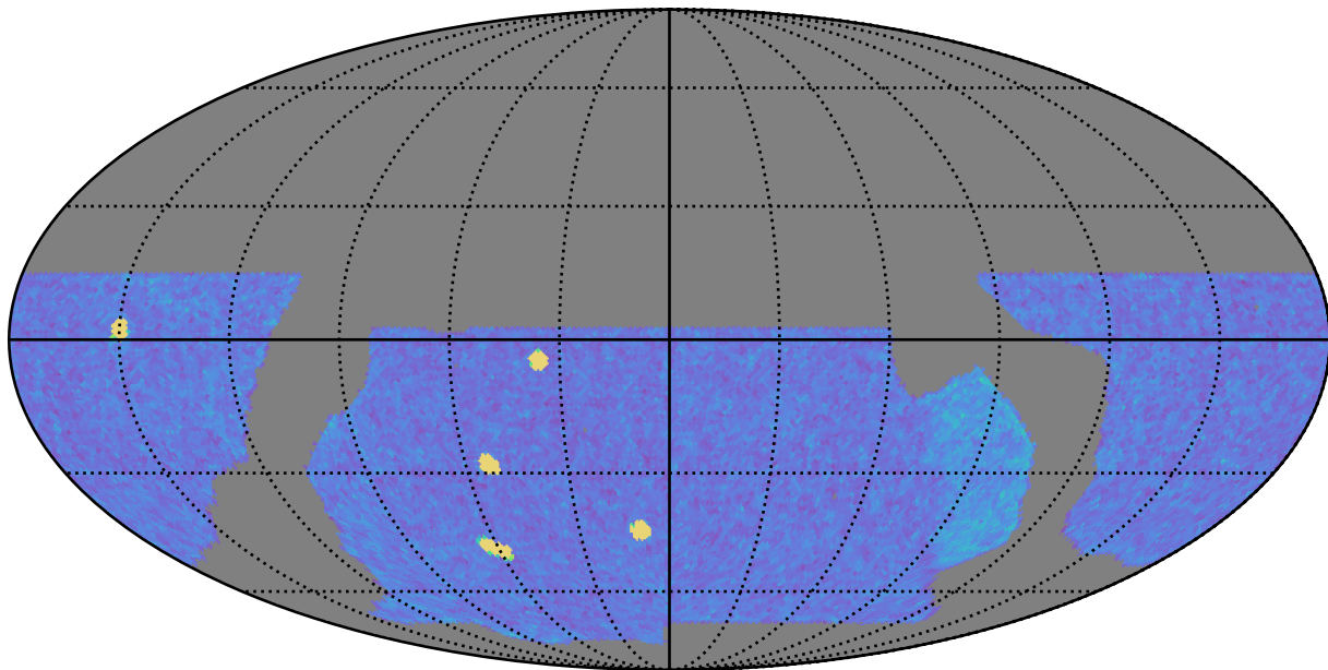
baseline_v2.0_10yrs WFD z band: NVisits
