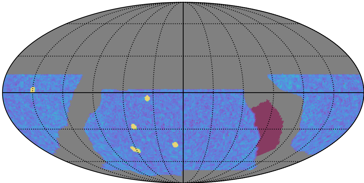
baseline_v2.0_10yrs WFD y band: NVisits
