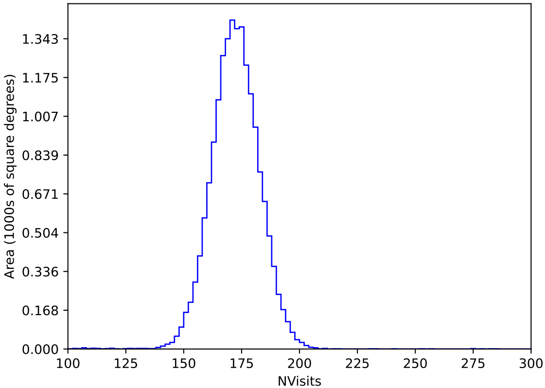
baseline_v2.0_10yrs WFD y band: NVisits
