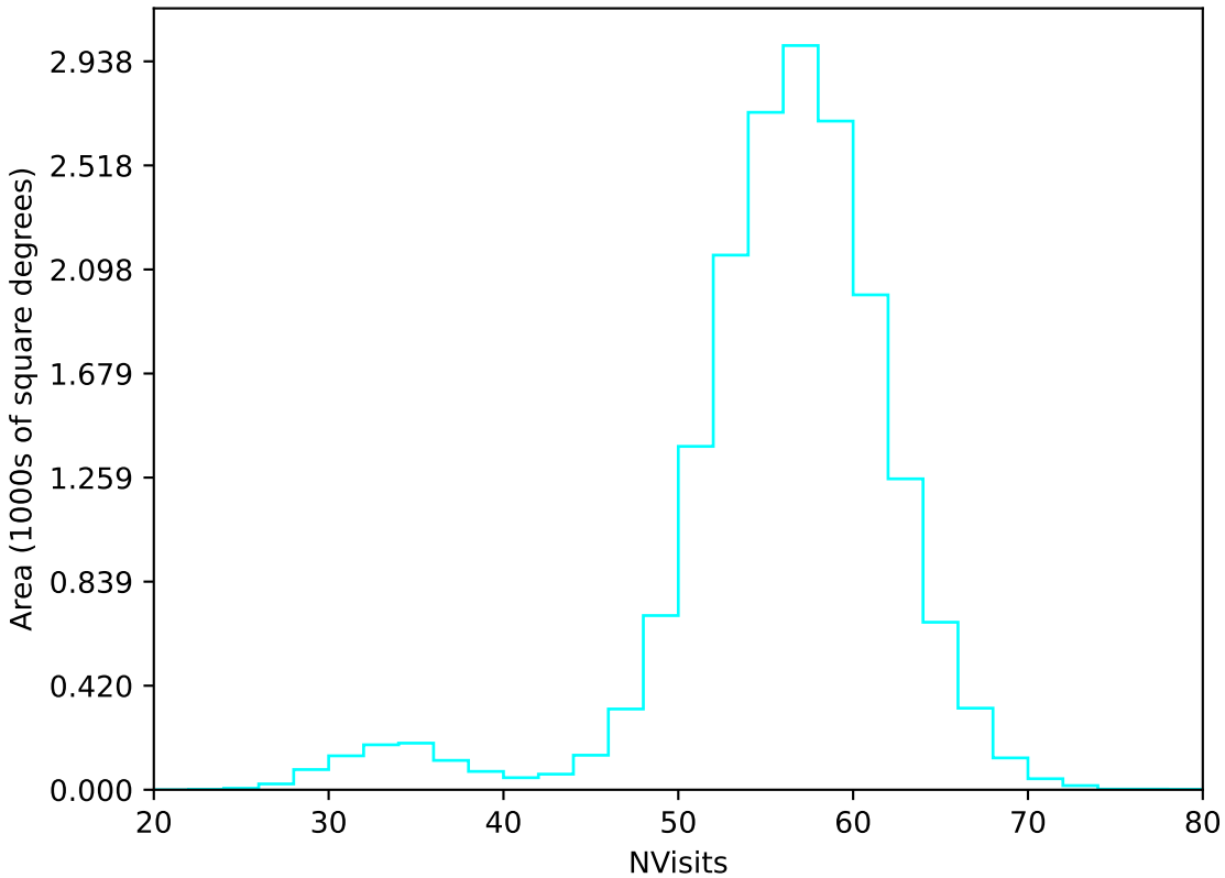
baseline_v2.0_10yrs WFD u band: NVisits
