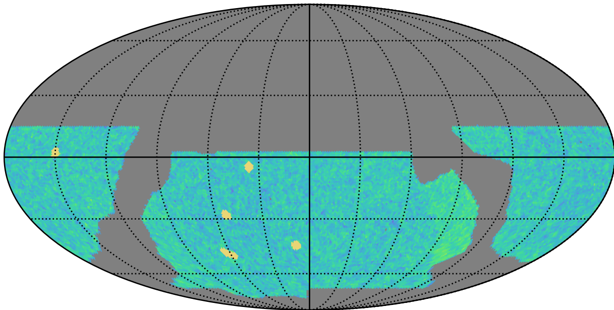
baseline_v2.0_10yrs WFD r band: NVisits
