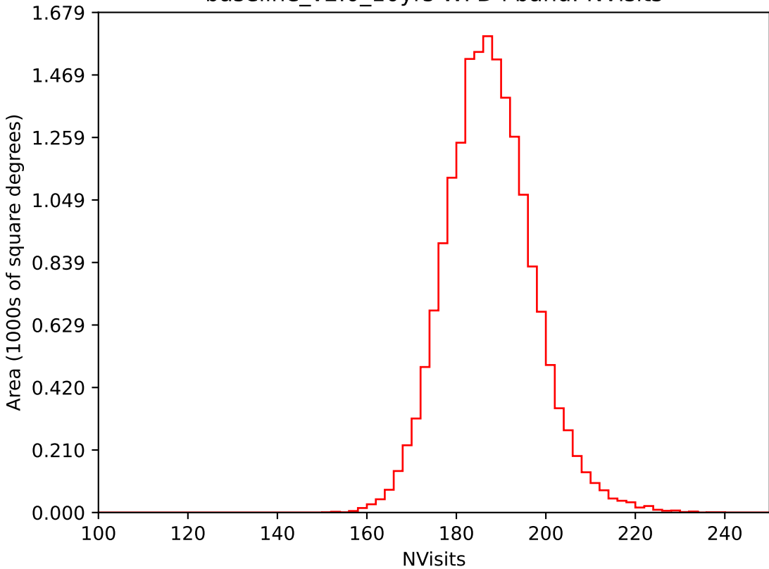
baseline_v2.0_10yrs WFD i band: NVisits
