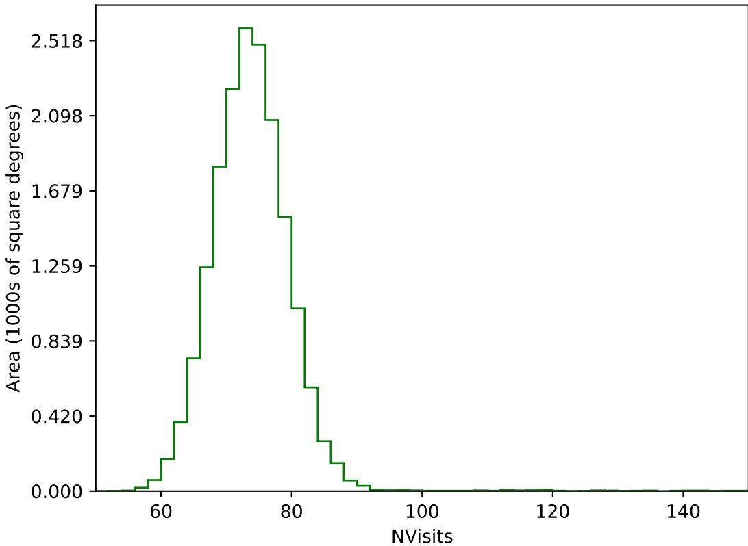
baseline_v2.0_10yrs WFD g band: NVisits
