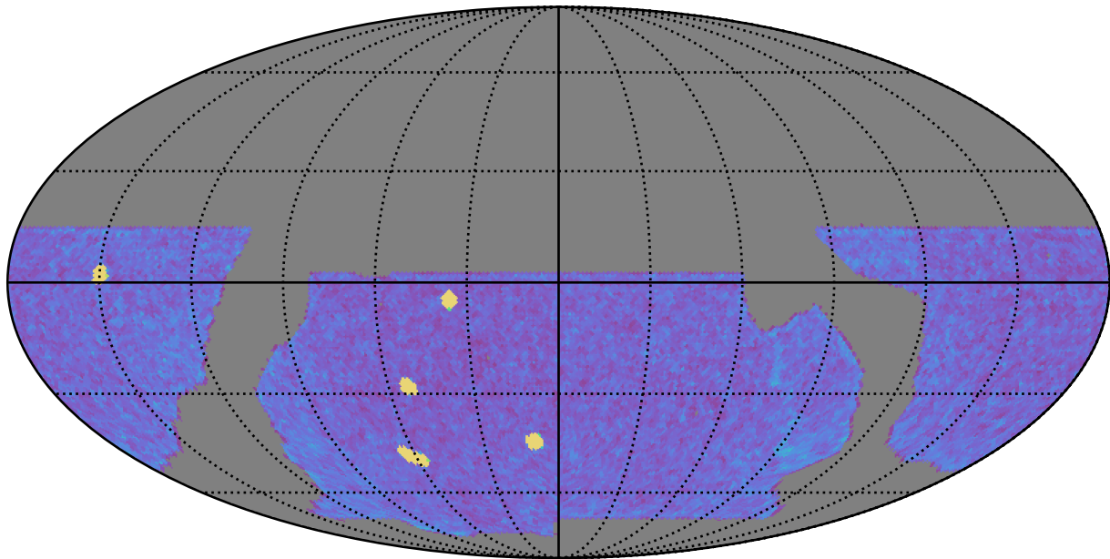
baseline_v2.0_10yrs WFD all bands: NVisits
