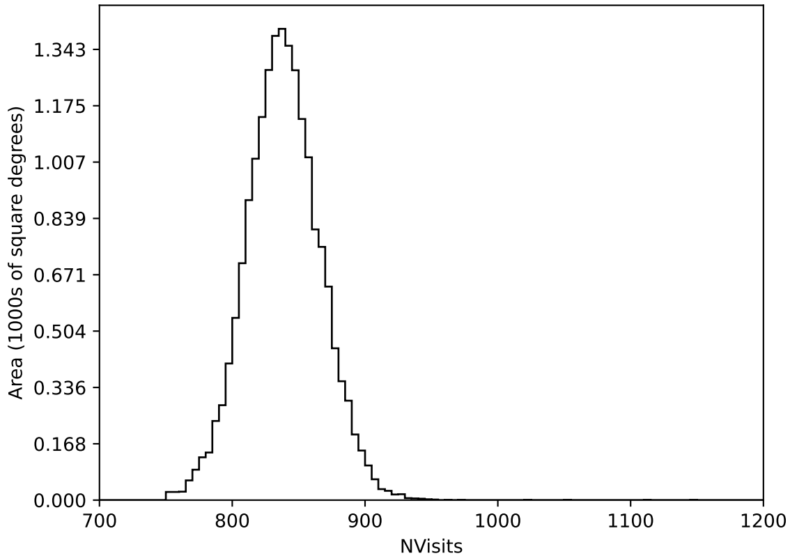
baseline_v2.0_10yrs WFD all bands: NVisits
