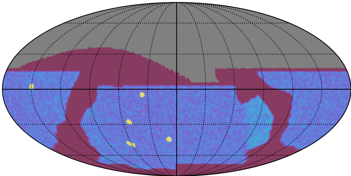
baseline_v2.0_10yrs All sky z band: NVisits
