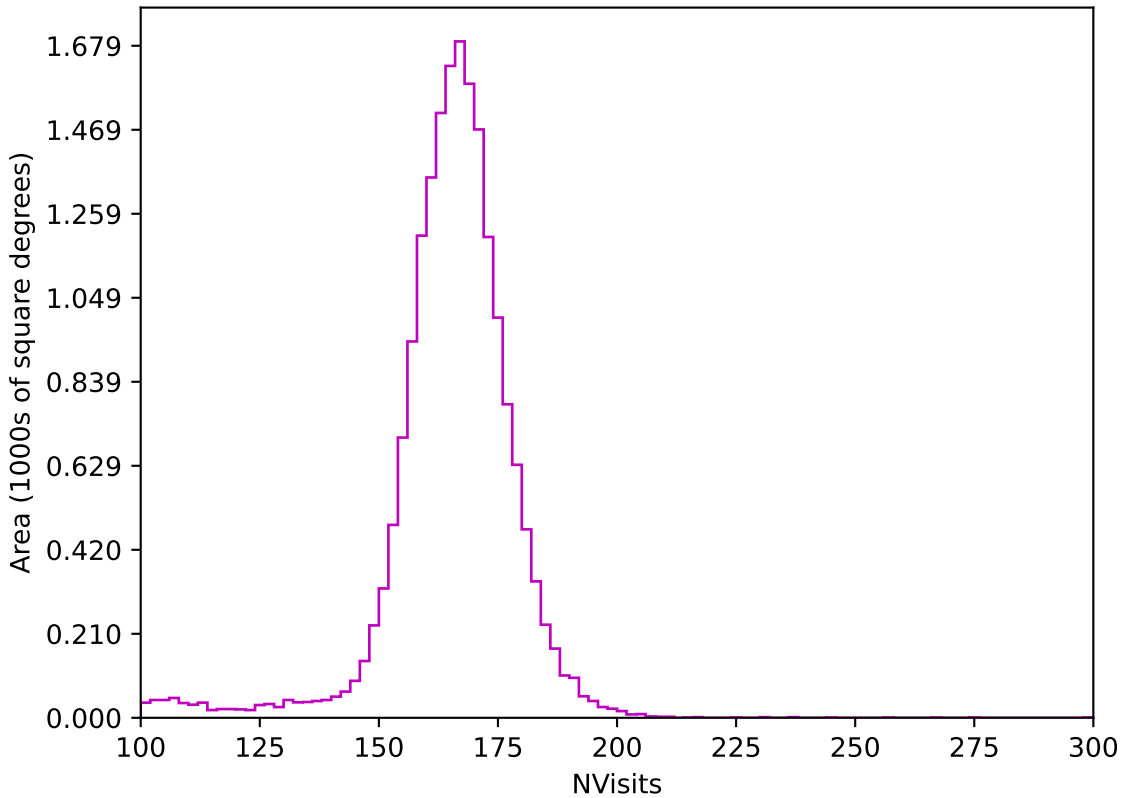
baseline_v2.0_10yrs All sky z band: NVisits
