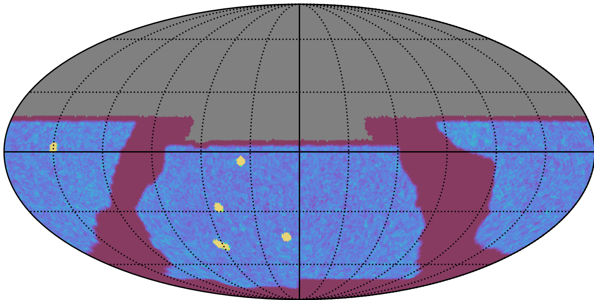
baseline_v2.0_10yrs All sky y band: NVisits
