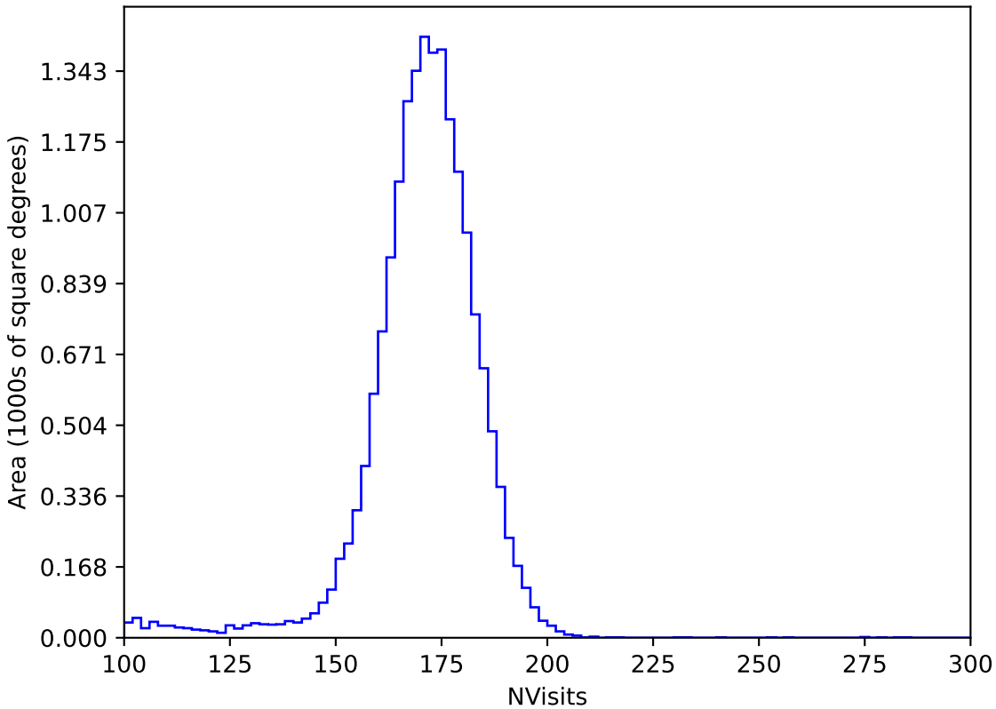
baseline_v2.0_10yrs All sky y band: NVisits
