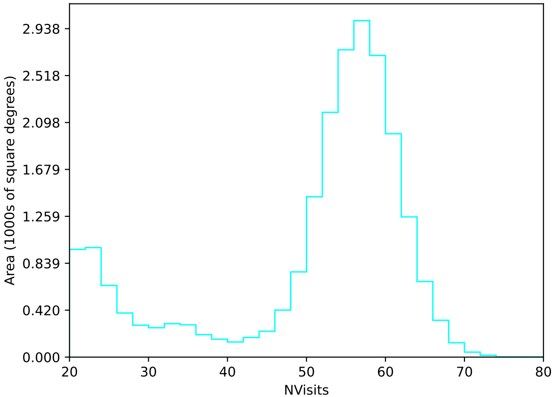
baseline_v2.0_10yrs All sky u band: NVisits
