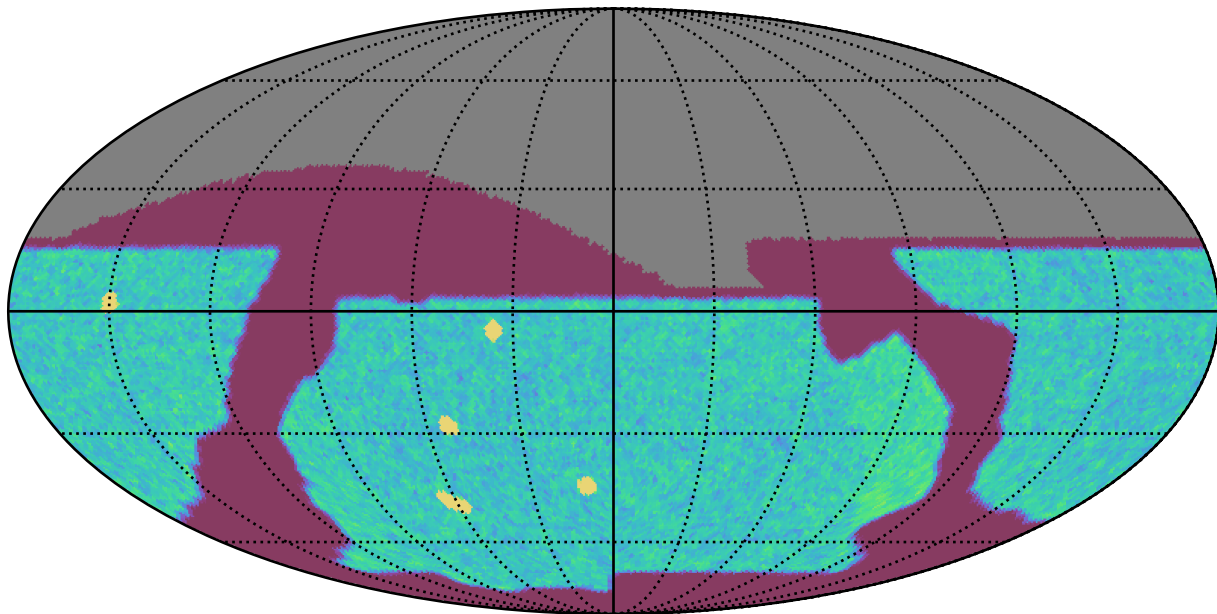
baseline_v2.0_10yrs All sky r band: NVisits
