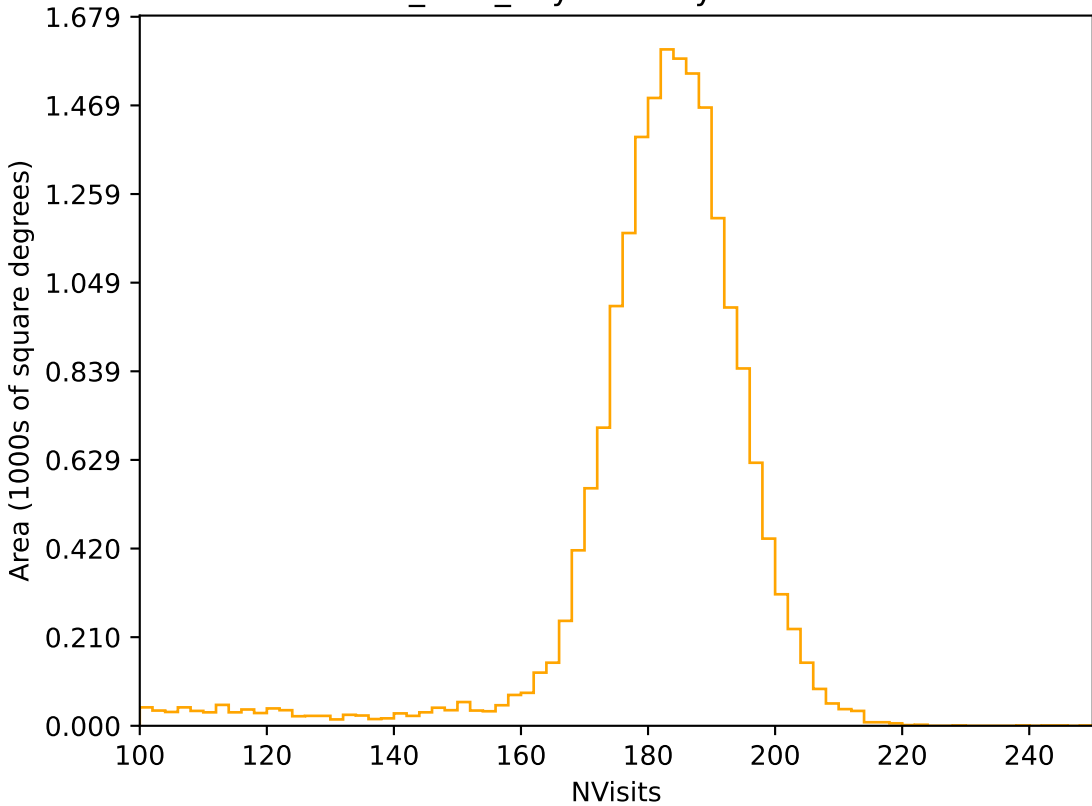
baseline_v2.0_10yrs All sky r band: NVisits
