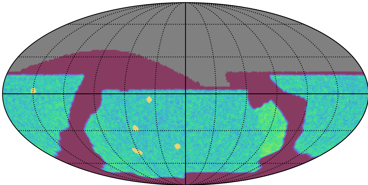
baseline_v2.0_10yrs All sky i band: NVisits
