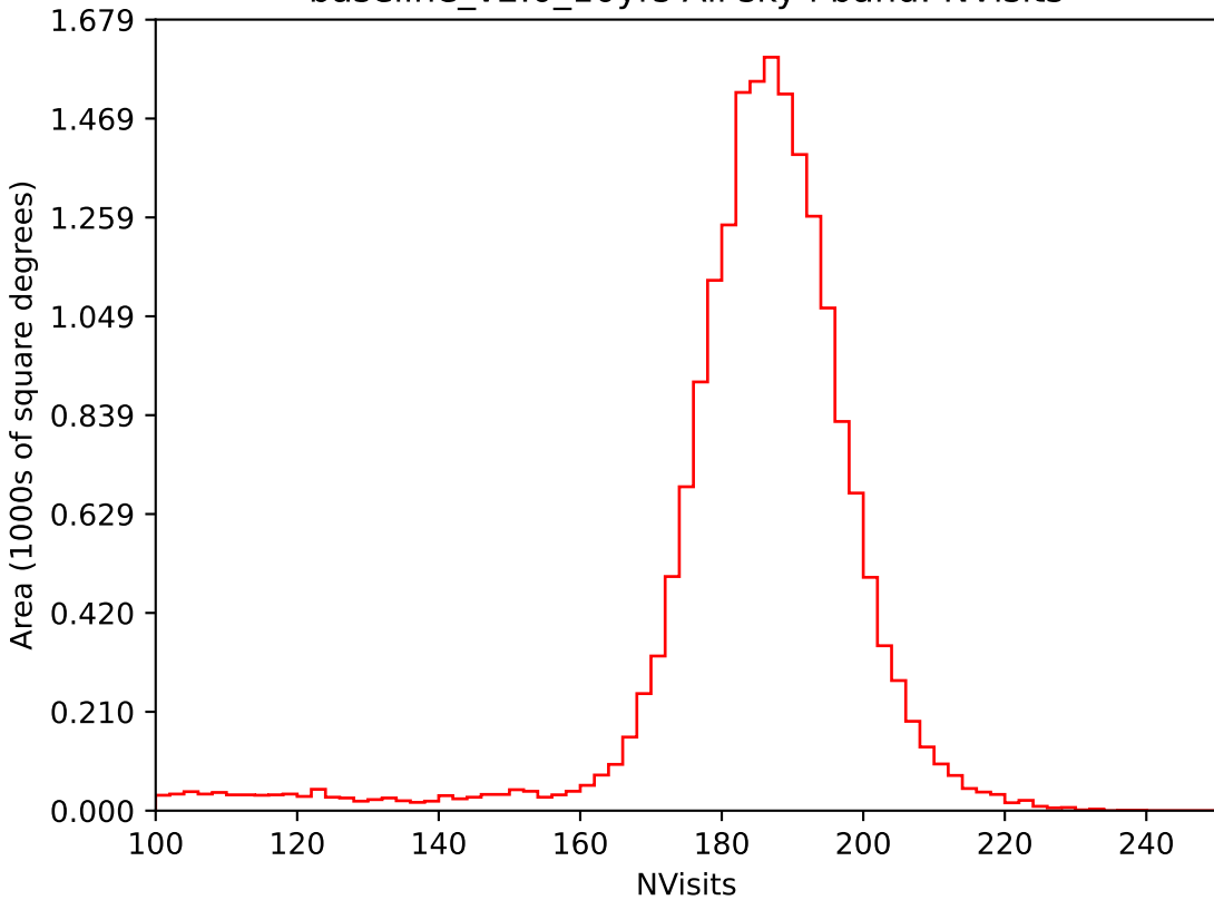
baseline_v2.0_10yrs All sky i band: NVisits
