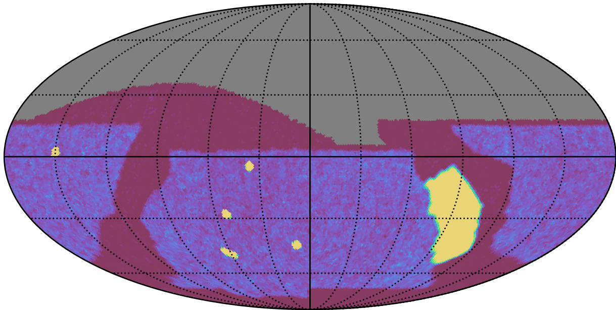
baseline_v2.0_10yrs All sky g band: NVisits
