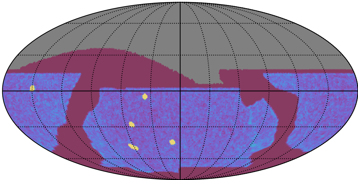
baseline_v2.0_10yrs All sky all bands: NVisits
