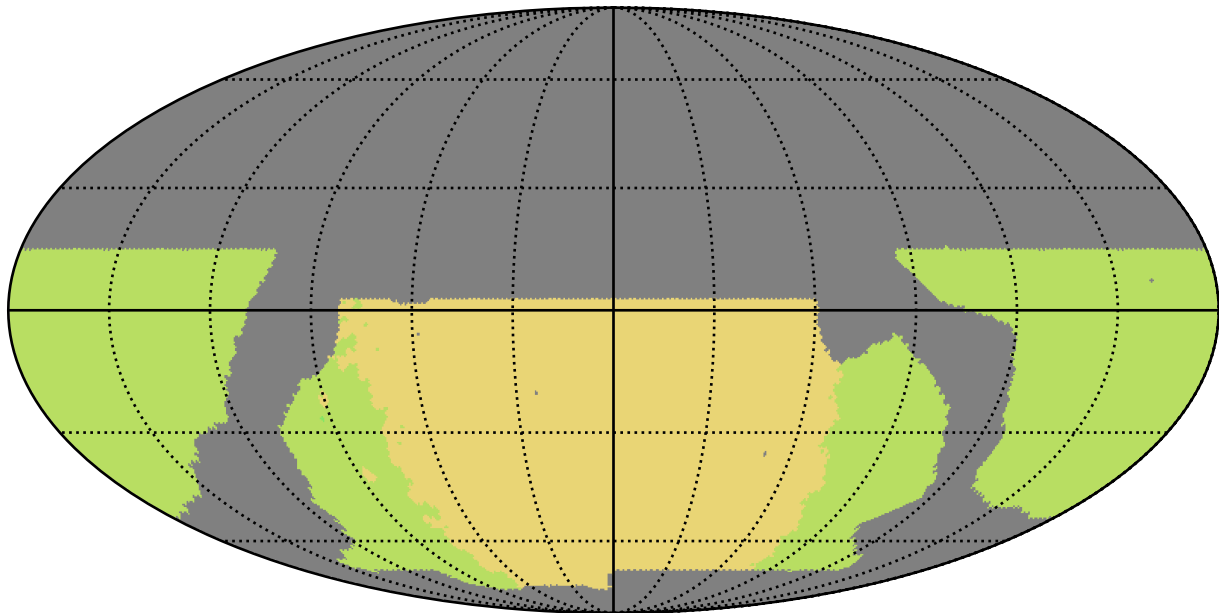
baseline_v2.0_10yrs WFD all bands: NSeasons
