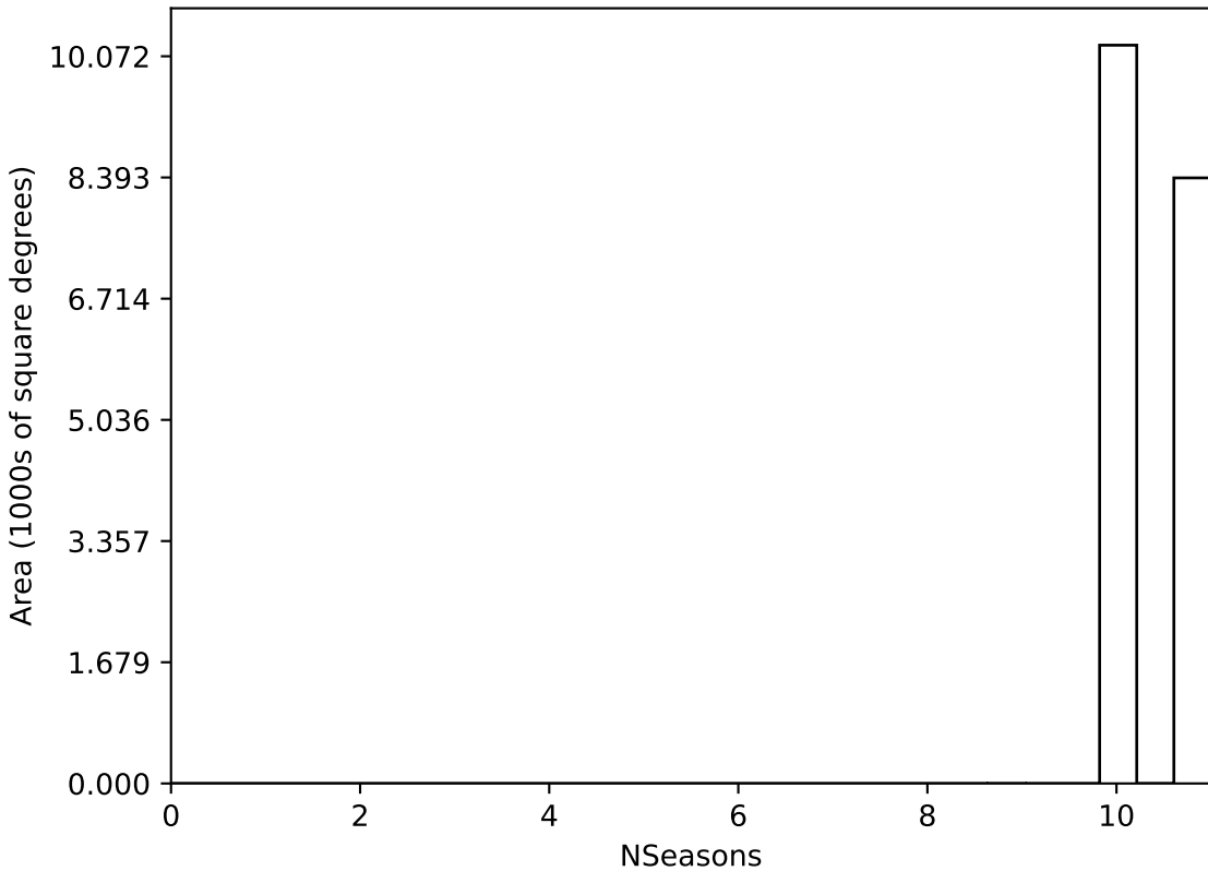
baseline_v2.0_10yrs WFD all bands: NSeasons
