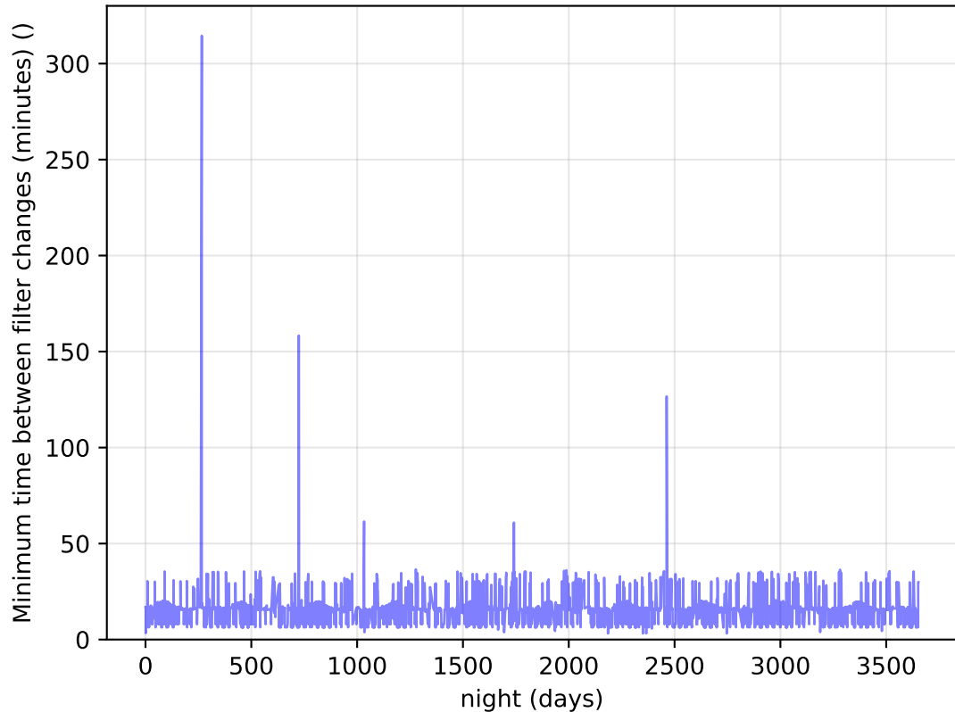
baseline_v2.0_10yrs Per Night: Minimum time between filter changes (minutes)
