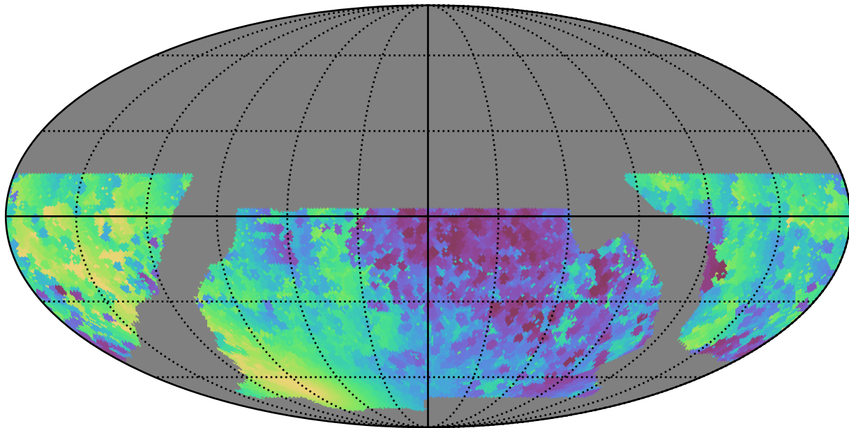
baseline_v2.0_10yrs WFD z band: Min solarElong
