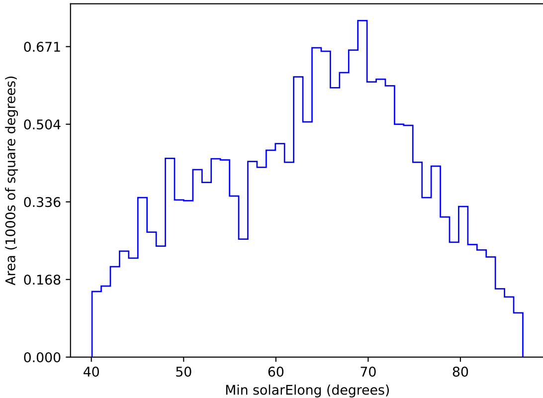
baseline_v2.0_10yrs WFD z band: Min solarElong
