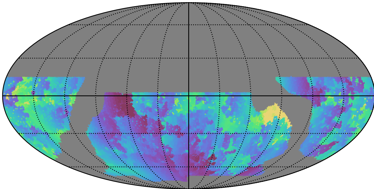
baseline_v2.0_10yrs WFD u band: Min solarElong
